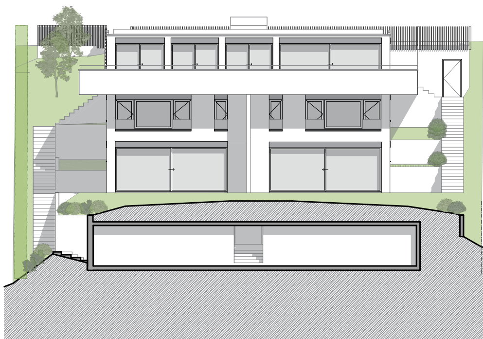
FACADE SUD BATIMENT A
