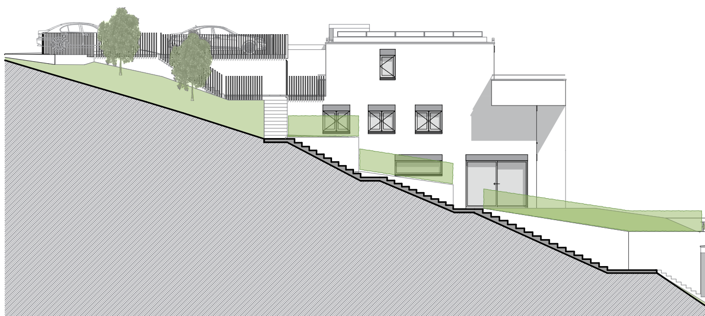
FACADE OUEST BATIMENT A
